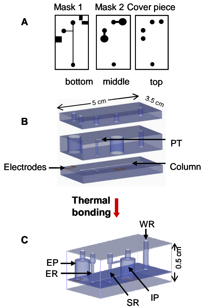
Figure 3.1. Schematics of the fabrication process to integrate micropumps with microchannels for microchip LC ( drawings not to scale, specific details in the text ). (A) Two masks are used to pattern the microchannels and micropumps in the bottom and middle layers. (B) Alignment of layers. (C) The final device containing sample and eluent pumps integrated with microchannels is formed by thermally bonding all the pieces together.
