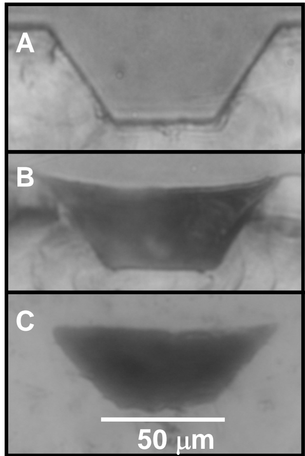
Figure 4.3 Edge-on photomicrographs of channel cross-sections at different fabrication stages. (A) Imprinted channel. (B) Imprinted channel filled with solidified PCSL. (C) Bonded device after PCSL removal. Reprinted with permission from ref. 37; copyright 2005, American Chemical Society.
