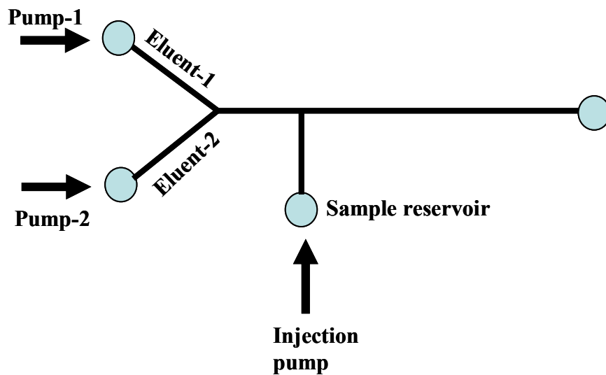
Figure 7.1 Layout of a microchip LC device with gradient elution capabilities.
