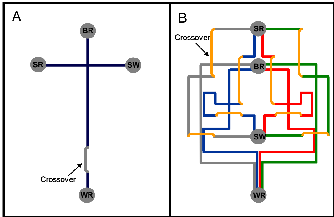
Figure 6.2 Microchip designs. (A) Microfluidic device for separations in crossover channels.
