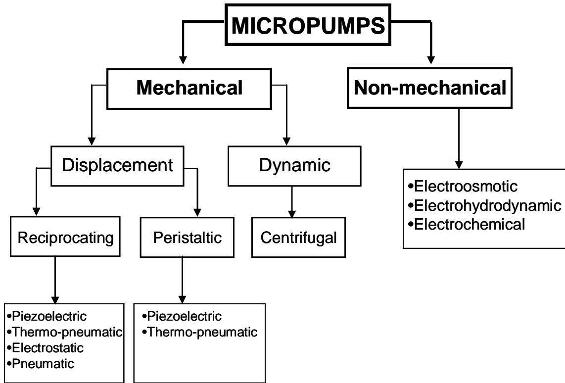
Figure 1.18. Micropump classification.
