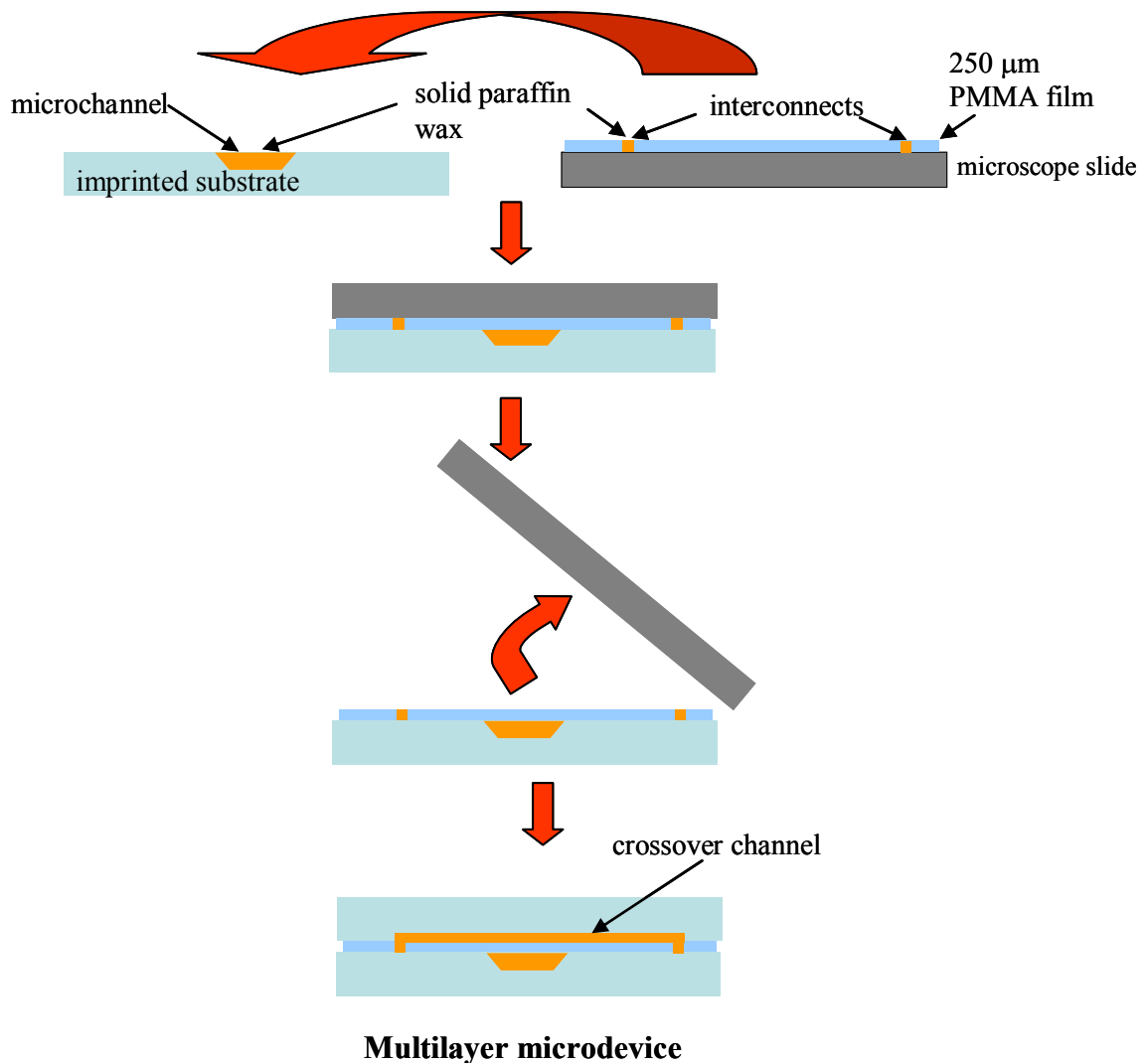
Figure 6.1 Schematic of the fabrication of multilayer microfluidic devices with a thin intermediate layer.
